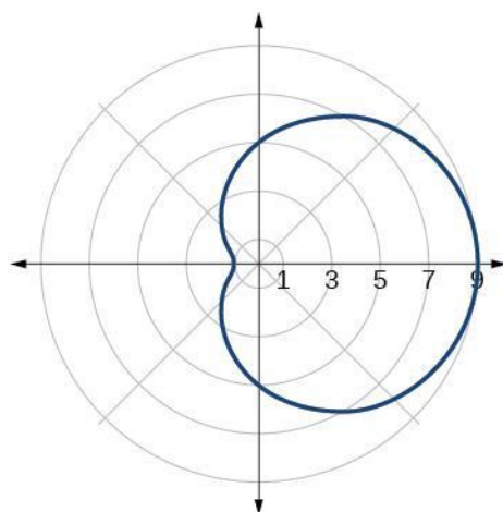
11. one-loop/dimpled limaçon
